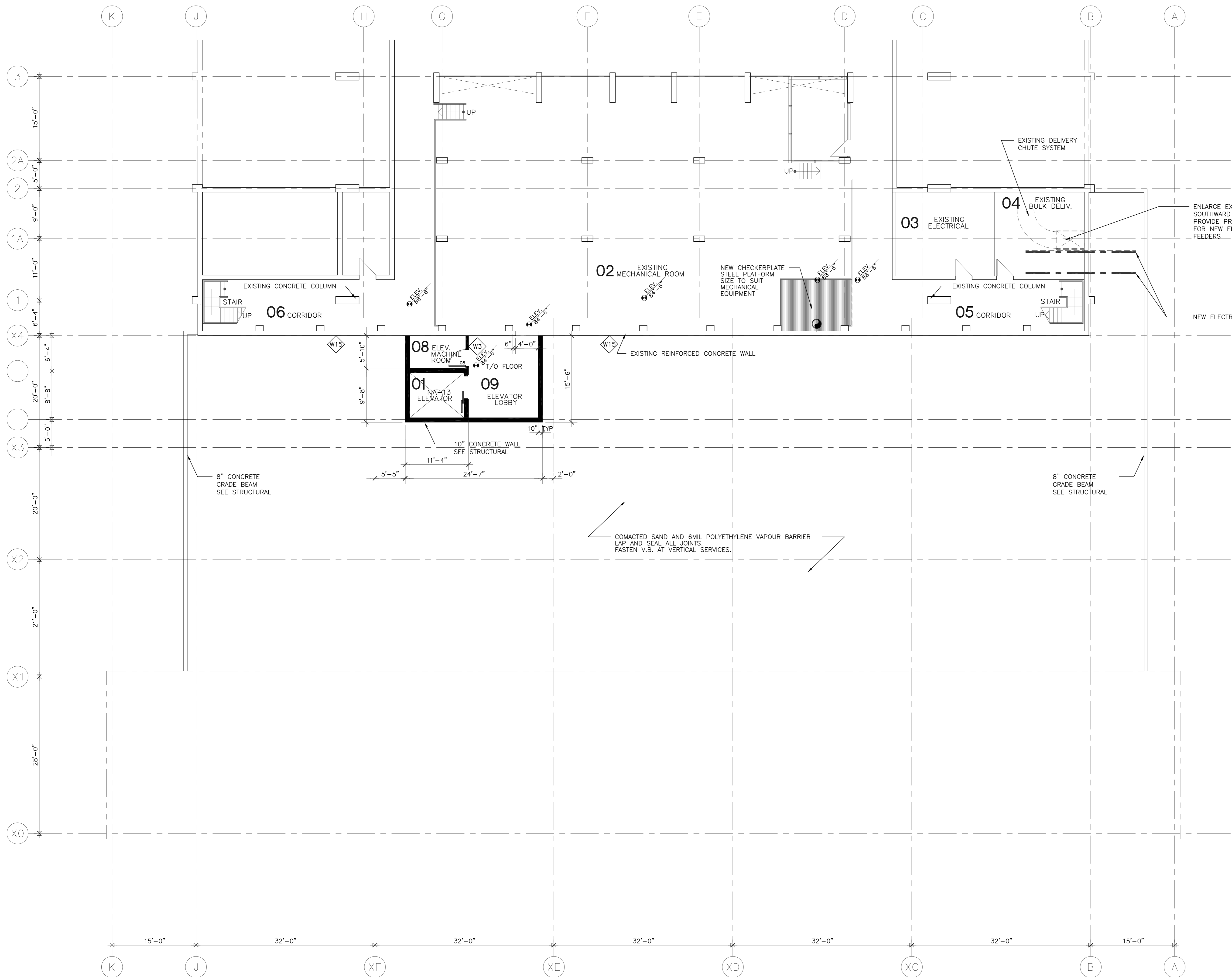
1 BASEMENT PLAN 1/8"=1'-0"
